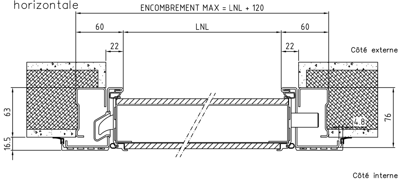
Section verticale
